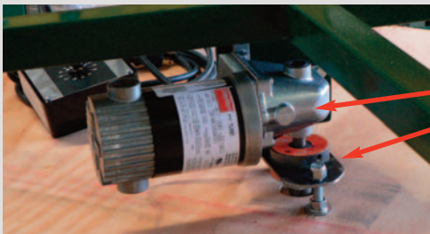
Inverted view of turn table drive
