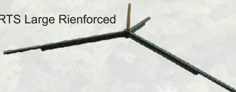
Large Reinforced Golden Spike 5/8" spike, 5/8" rebar, 22" legs
